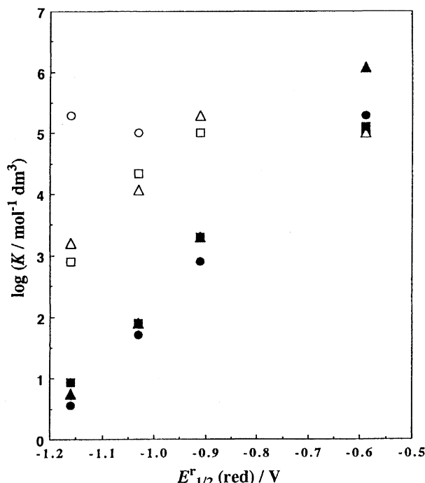
Fig. 3. Correlation between E_{1/2}^{\circ}(\text{red}) of metalladithiolene complexes and equilibrium constant K for the adduct formation with phosphine and phosphite.
