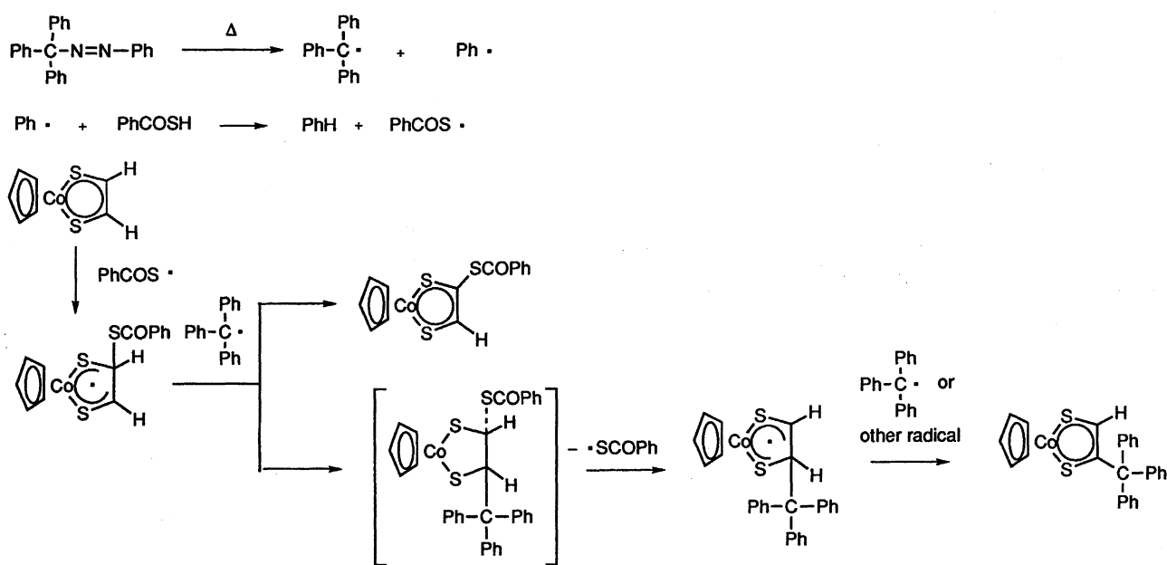
Scheme 7.
