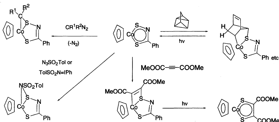
Scheme 11.
