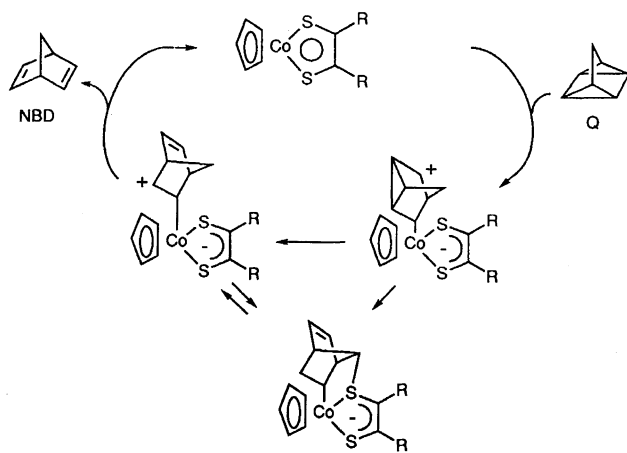
Scheme 33.
