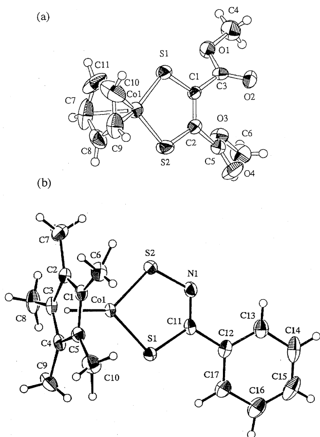
Fig. 1. X-Ray structures of a cobaltadithiolene, [(\text{Cp})\text{Co}\{\text{S}_2\text{C}_2(\text{COOMe})_2\}] , and a cobaltadithiazole, [(\text{Cp}^*)\text{Co}(\text{S}_2\text{CNPh})] .
